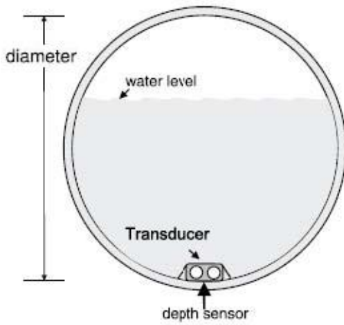
Partially pipe
