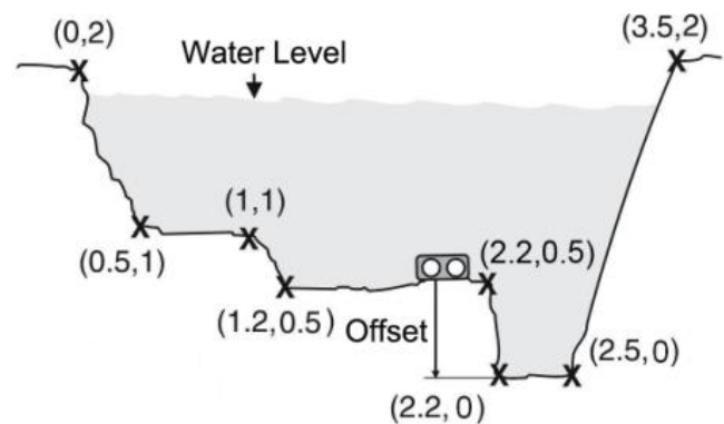
Irregular-shaped channel
